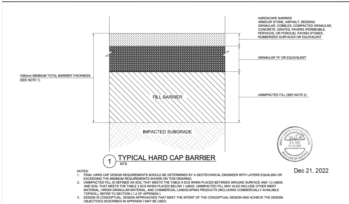
FIGURE I-1 Conceptual Design of Typical Hard Cap Barrier (City Parks)
