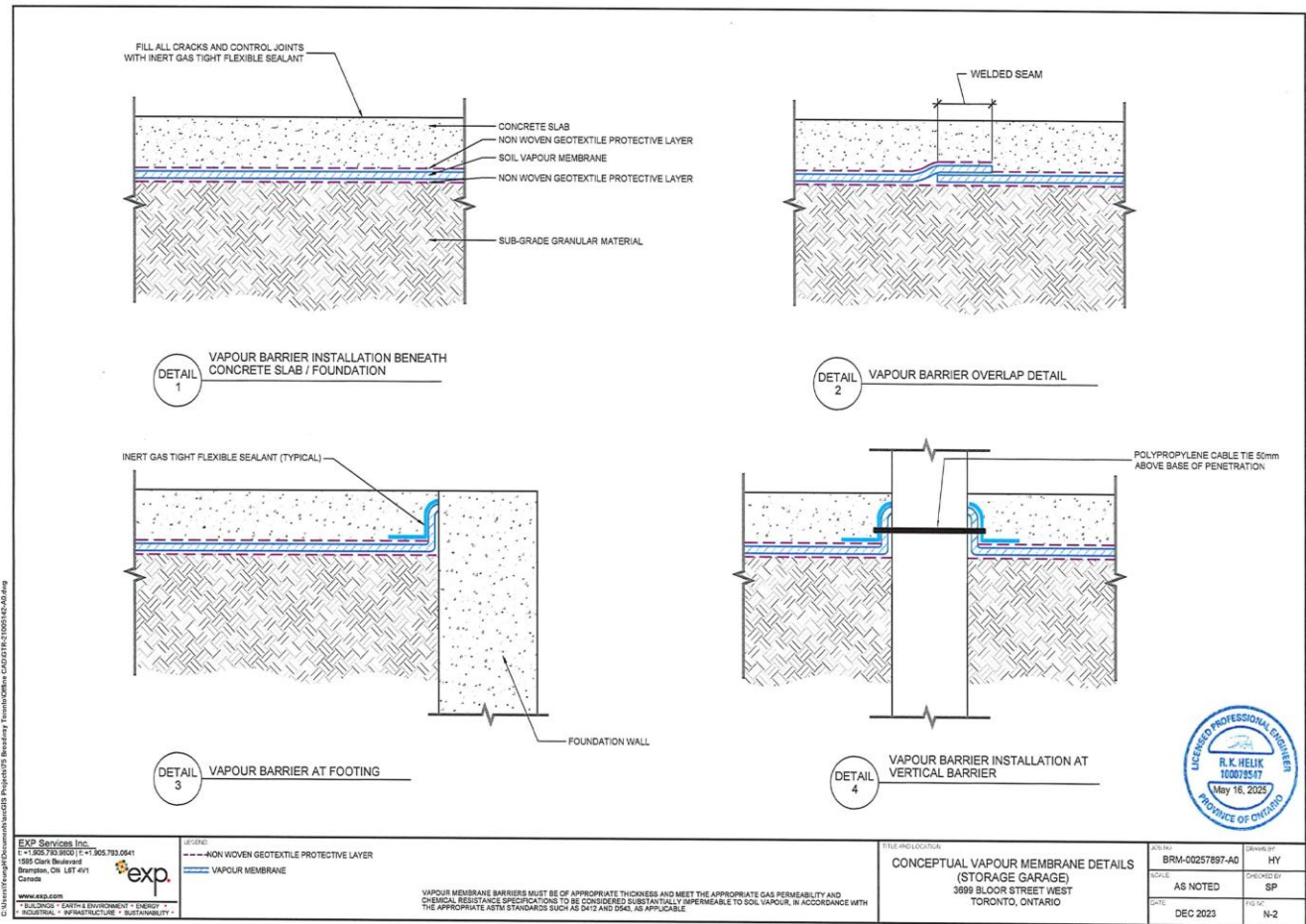
Figure N-2
